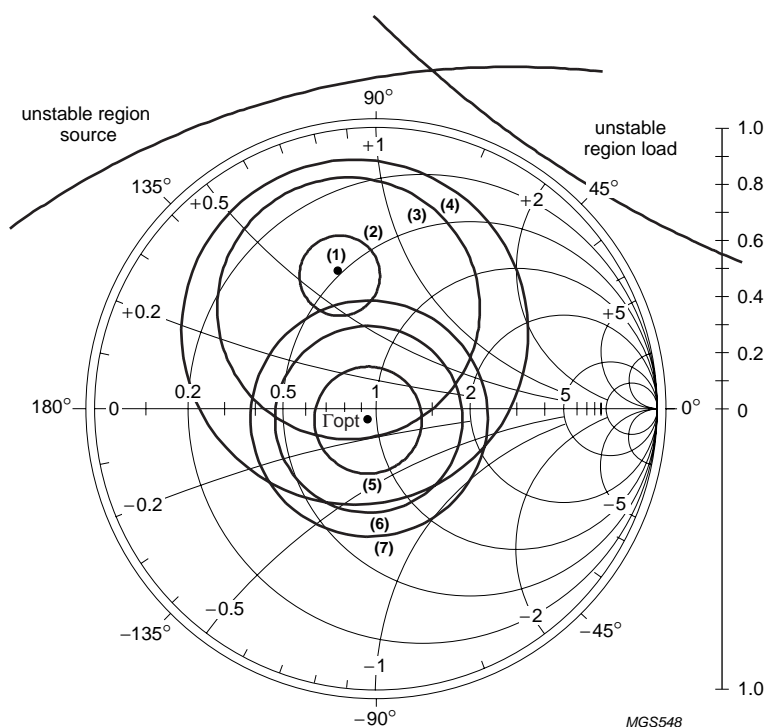
Fig.14 Noise, stability and gain circles; typical values.
