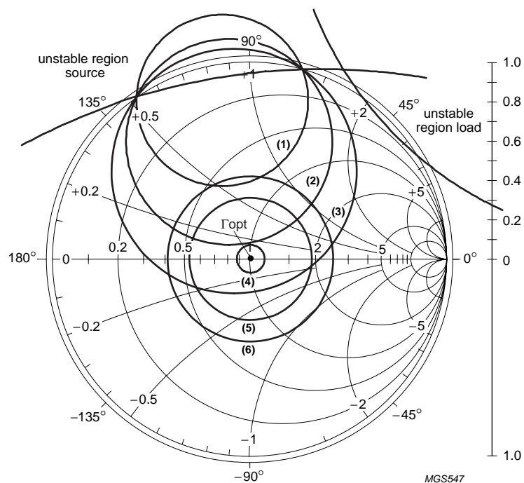
Fig.13 Noise, stability and gain circles; typical values.
