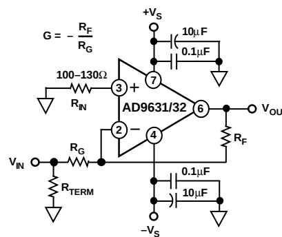
Figure 58. Inverting Operation
