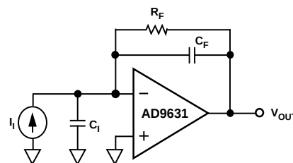
Figure 59. Transimpedance Configuration
