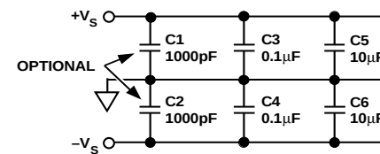
Supply Bypassing
