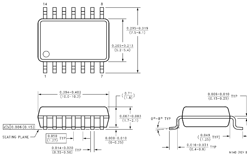
14-Lead Molded Small Outline Package, EIAJ Package Number M14D
