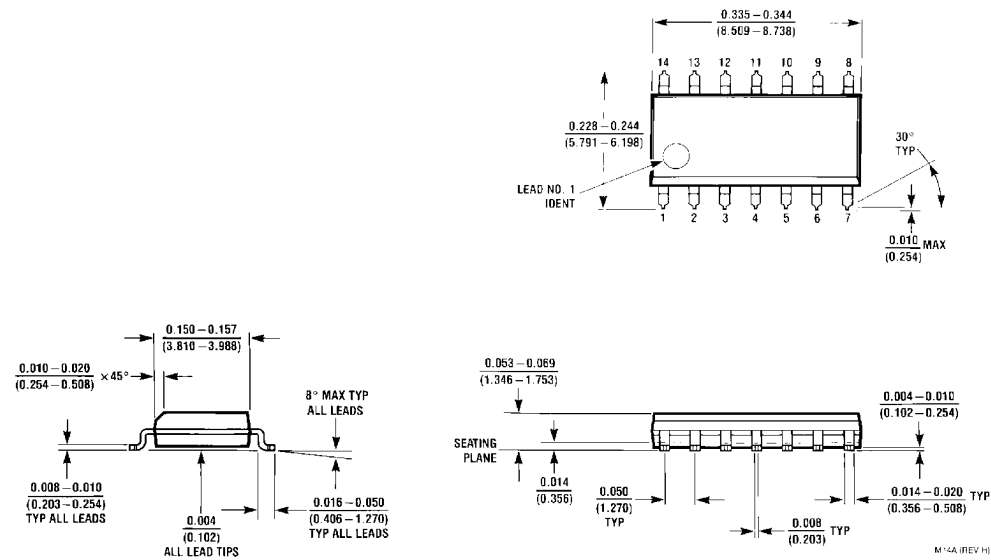
14-Lead (0.50" Wide) Molded Small Outline Package, JEDEC Package Number M14A
