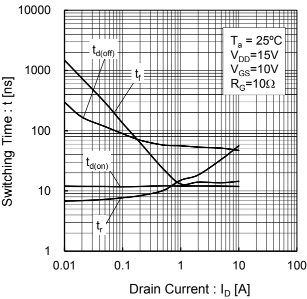
Fig.19 Switching Characteristics
