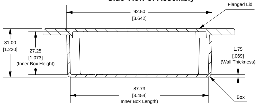
SECTION B-B Side View of Assembly
