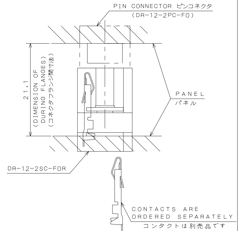
MATED CONDITION (REF.) 嵌合状態図 (参考)
