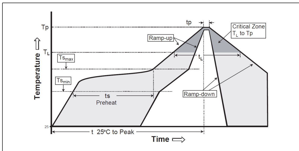
Figure 34: Soldering Recommendations
