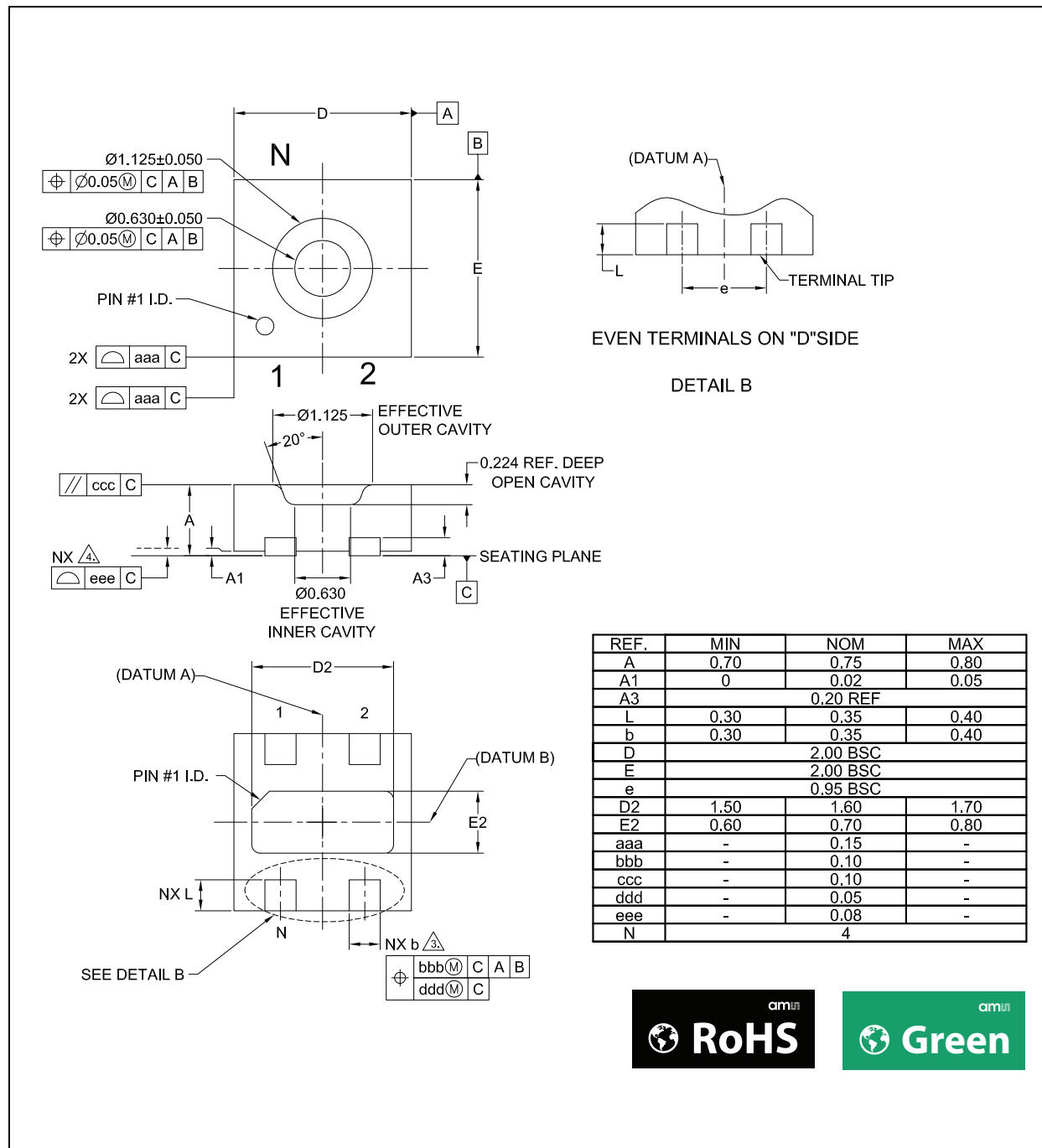
Figure 37: Package Outline
