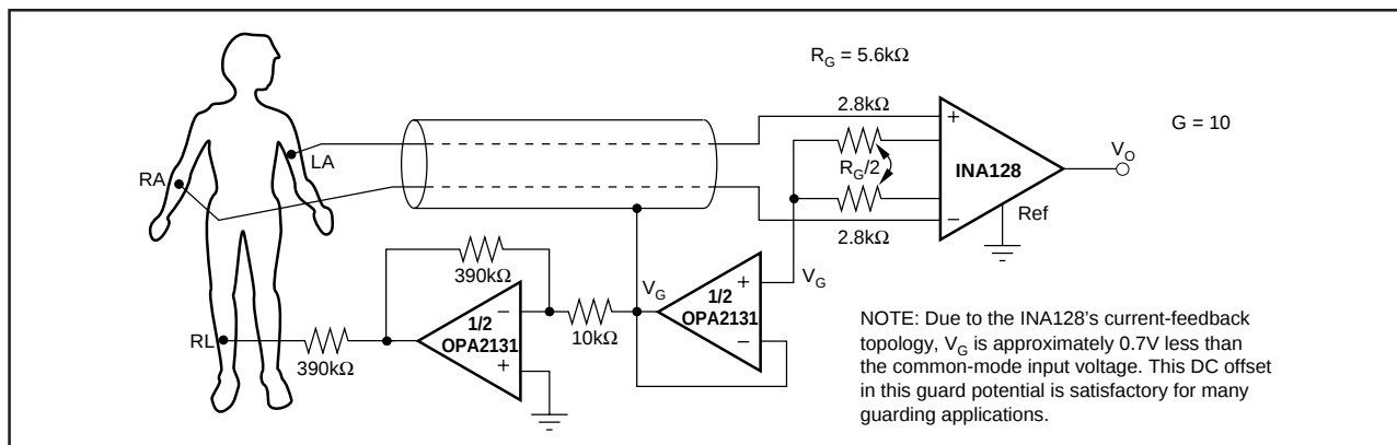
FIGURE 4. ECG Amplifier With Right-Leg Drive.
