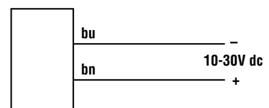
Quick-Disconnect hookup
