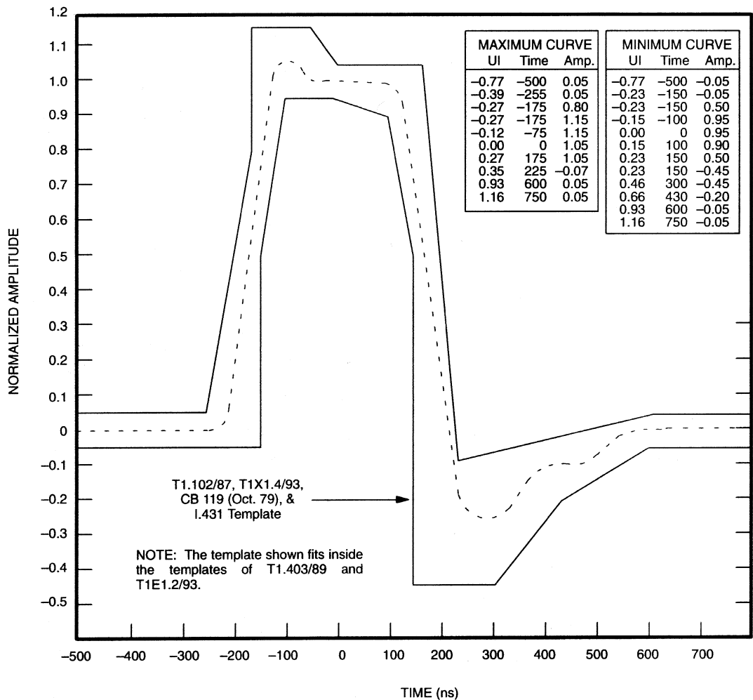
DS2151Q TRANSMIT WAVEFORM TEMPLATE Figure 12-3
