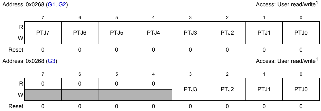
Figure 2-42. Port J Data Register (PTJ)
