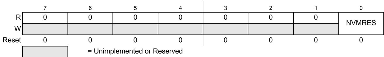
Figure 5-7. MMC Control Register (MMCCTL1)
