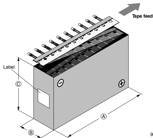
Fig. 41 - Tape Direction
