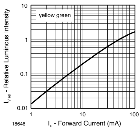
Fig. 29 - Relative Luminous Flux vs. Forward Current
