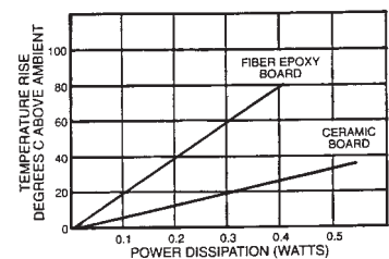
POWER DERATING
