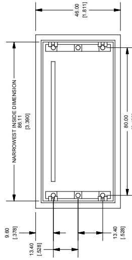
FRONT VIEW OF BOX
