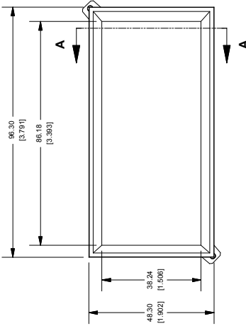
ASSEMBLED ENCLOSURE
