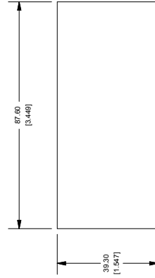
FACE PLATE (ALUMINUM)
