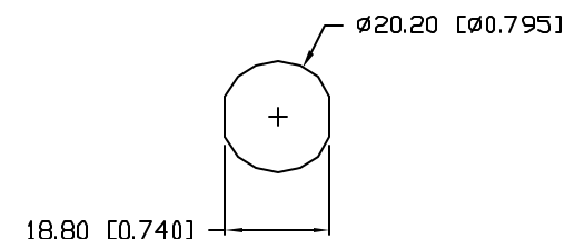
PANEL CUTOUT
