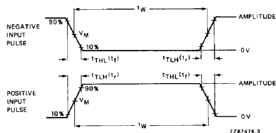
Fig. 21 Input pulse definitions.
