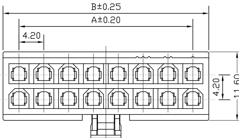
MF42-HF Female Housing
