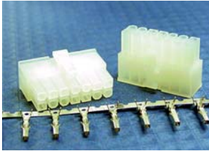
MF42-HF Female Housing
