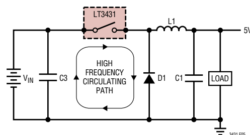
Figure 5. High Speed Switching Path
