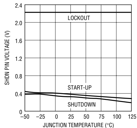
Lockout and Shutdown Thresholds
