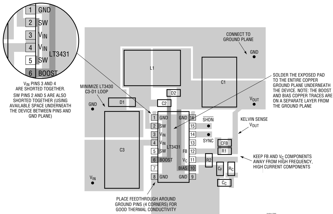
Figure 6. Suggested Layout
