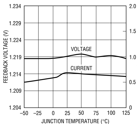
FB Pin Voltage and Current
