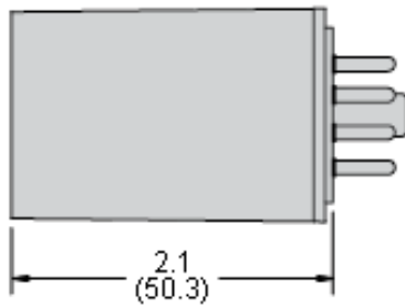
Plain Cover Dimensions
