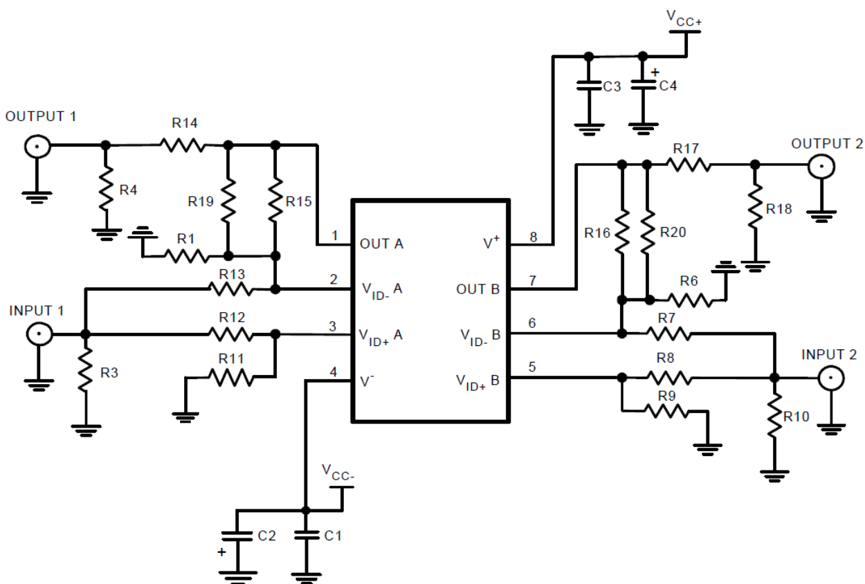
Figure 3: LMH730123 Schematic
