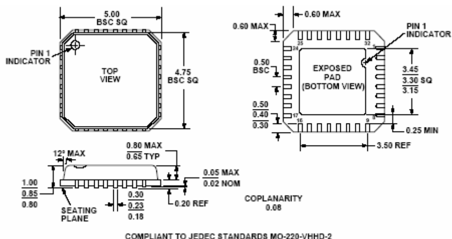
Figure 2. 32-Lead LFCSP
