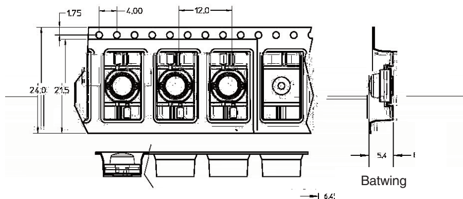
Figure 10. Tape dimensions for Batwing radiation pattern.
