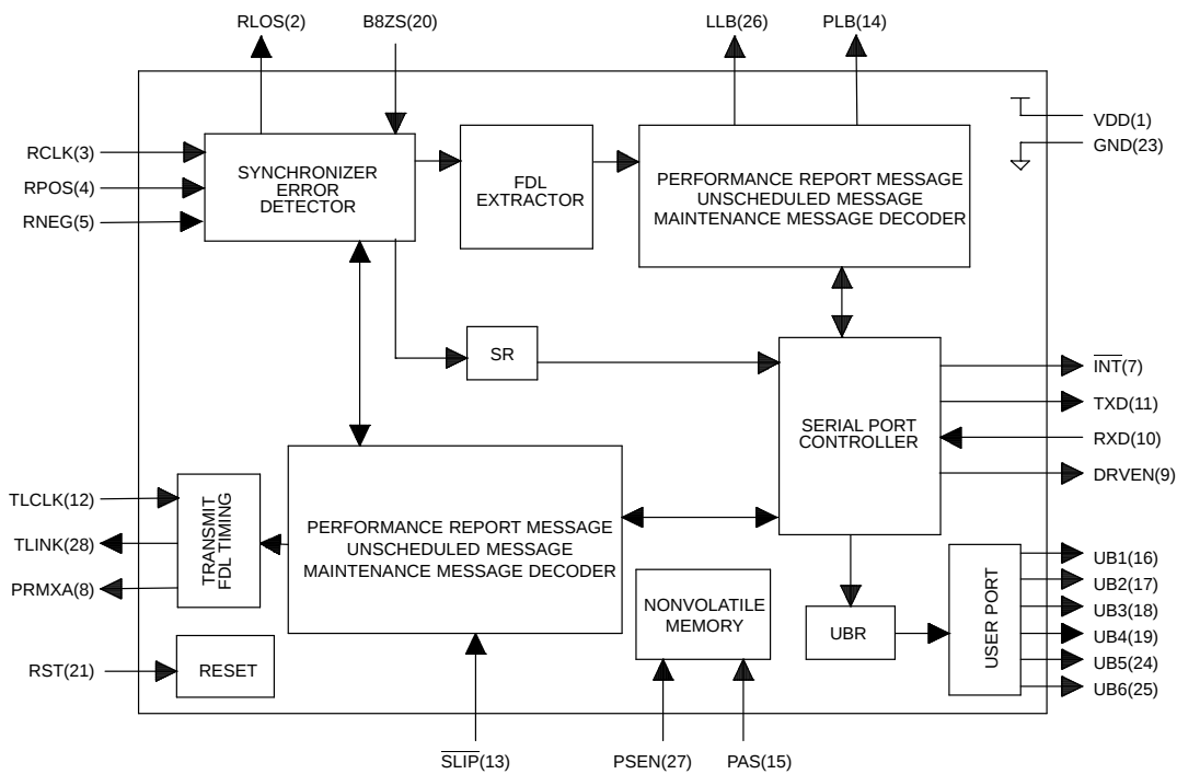
DS2282 BLOCK DIAGRAM Figure 1
