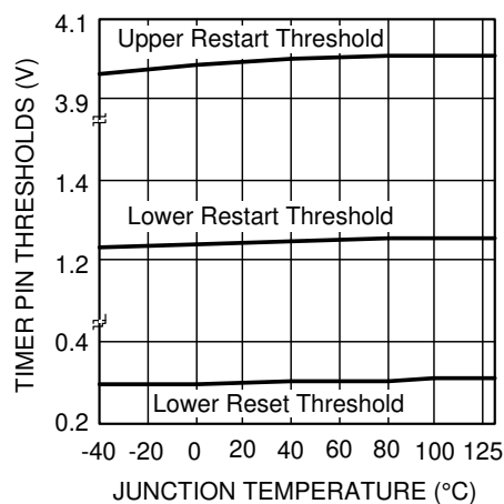
Figure 7-20. TIMER Pin Thresholds vs Temperature
