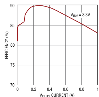
LV Channel Efficiency, 2MHz, V_{OUT2} = 1.8V
