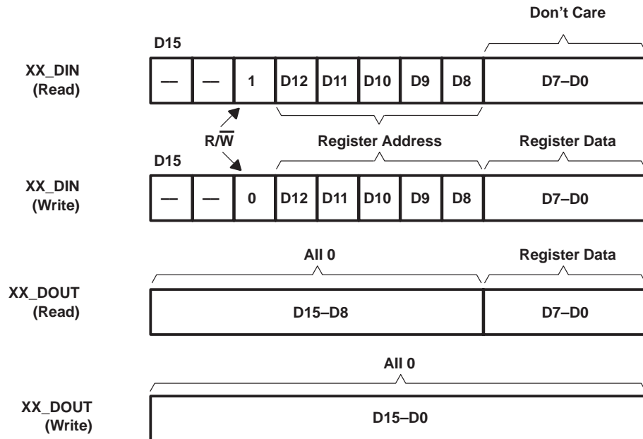
Figure 4–4. Secondary Communication DIN and DOUT Data Format
