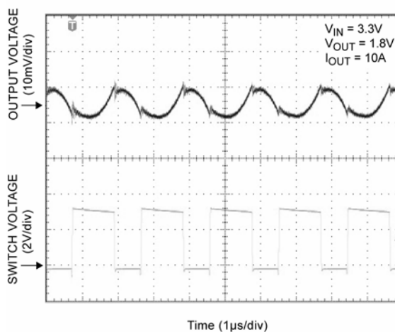
Operating Waveforms
