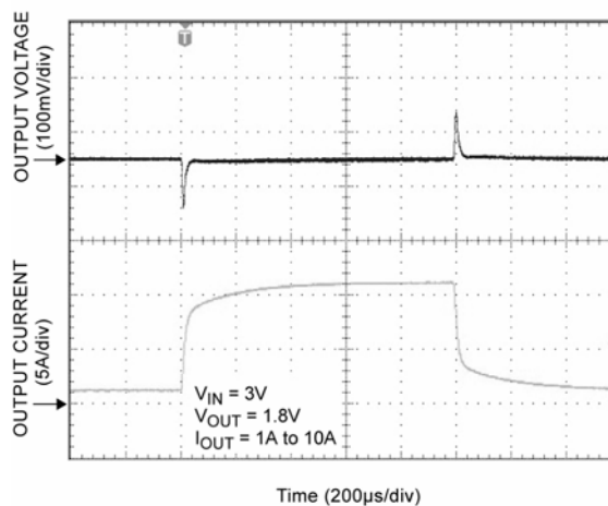
Operating Waveforms
