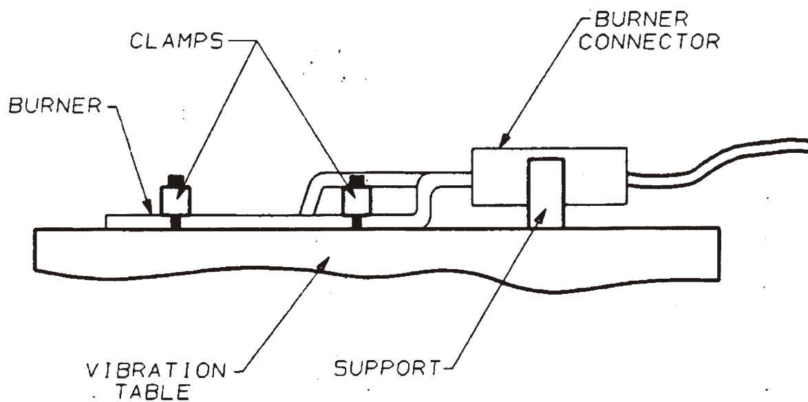
Figure 5 Mounting & Clamping Location For Vibration & Physical Shock
