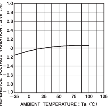
Fig.1 Reference voltage variation vs. ambient temperature
