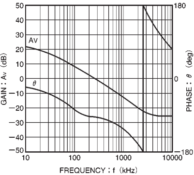
Fig.3 Gain and phase vs. frequency for the error amplifier (20 dB, close)
