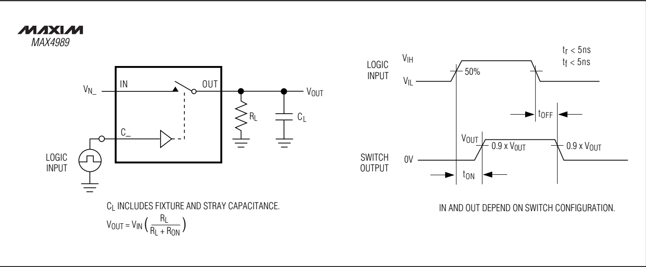
Figure 2. Switching Time
