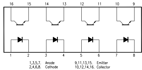
PIN NO. AND INTERNAL CONNECTION DIAGRAM
