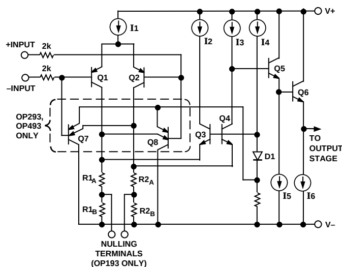
Figure 23. OP193/OP293/OP493 Equivalent Input Circuit
