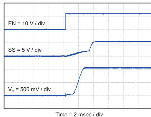
Figure 8. Start-up Waveform
