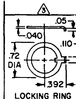
LOCKING RING
