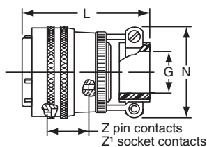
TERMINATION ASSEMBLIES “CE” (SR) Strain Relief
