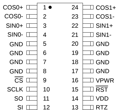
Figure 3. 33970 Pin Connections
