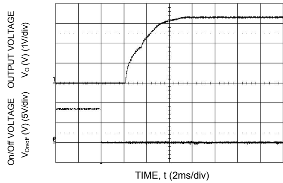
Figure 17. Typical Start-up Using Remote On/Off ( V_{IN} = V_{IN,NOM} , I_o = I_{o,max} ).
