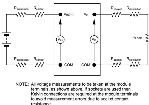
Figure 40. Output Voltage and Efficiency Test Setup.
