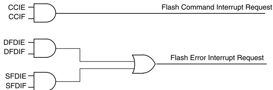
Figure 23-26. Flash Module Interrupts Implementation
