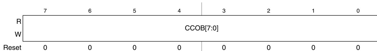
Figure 23-16. Flash Common Command Object Low Register (FCCOBLO)
