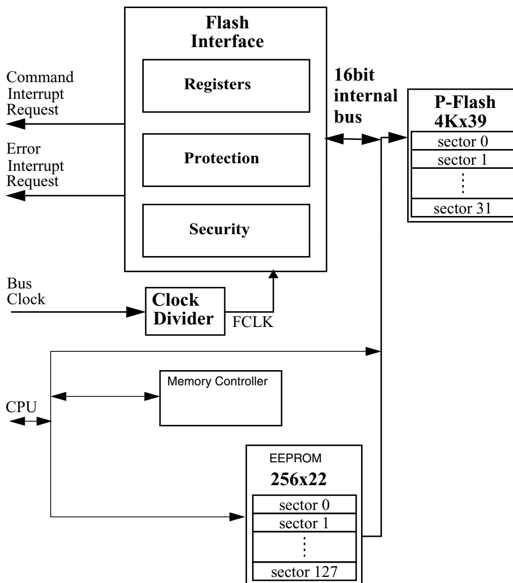
Figure 23-1. FTMRG16K1 Block Diagram
