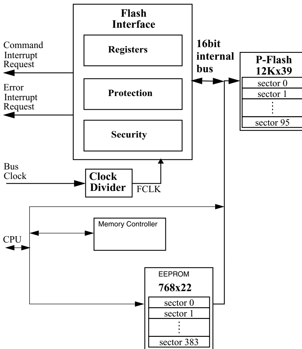
Figure 25-1. FTMRG48K1 Block Diagram
