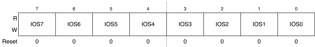
Figure 22-6. Timer Input Capture/Output Compare Select (TIOS)
