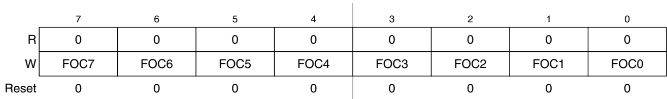
Figure 22-7. Timer Compare Force Register (CFORC)
