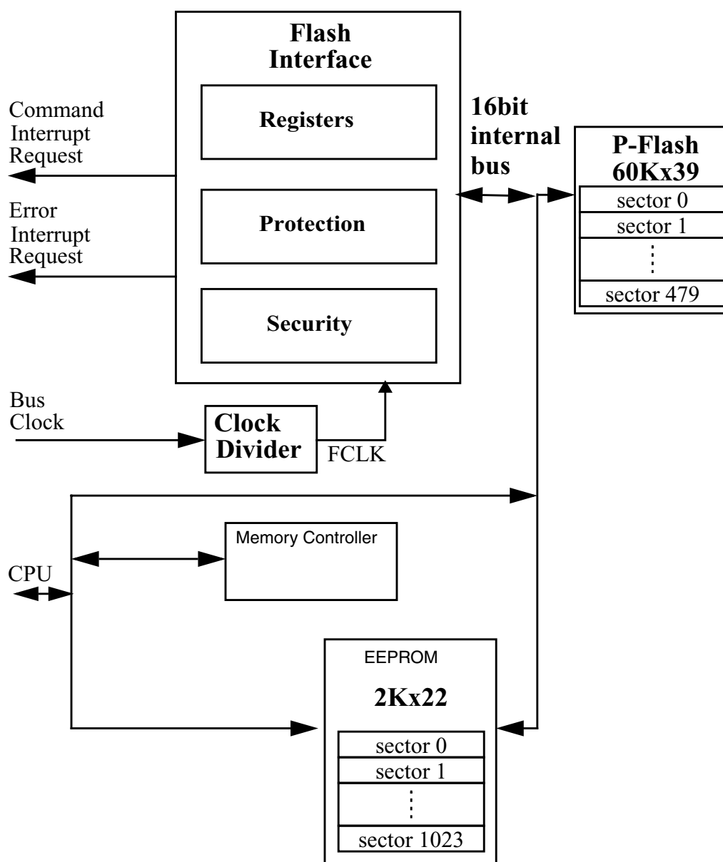
Figure 30-1. FTMRG240K2 Block Diagram
