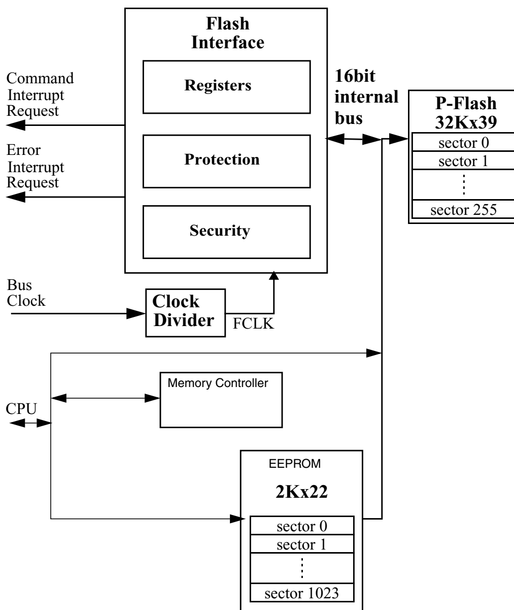
Figure 28-1. FTMRG128K1 Block Diagram
