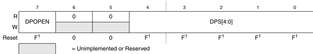
Figure 23-14. EEPROM Protection Register (EEPROT)
