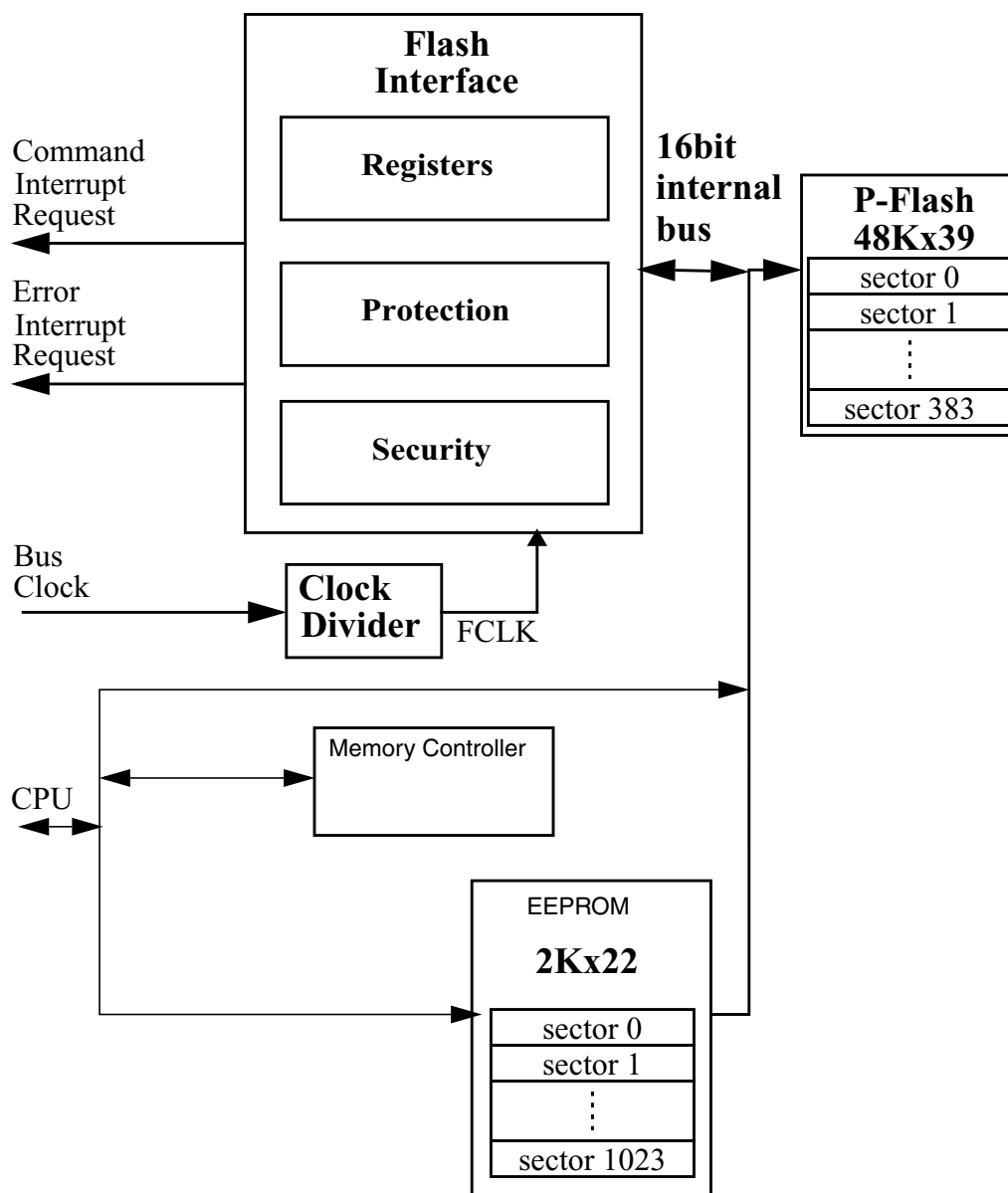
Figure 29-1. FTMRG192K2 Block Diagram
