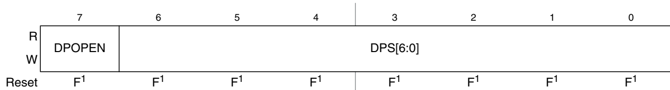
Figure 29-15. EEPROM Protection Register (EPROT)
