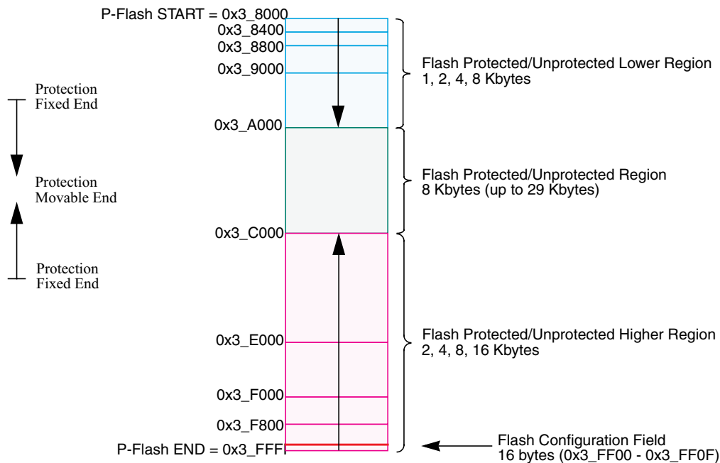
Figure 24-2. P-Flash Memory Map
