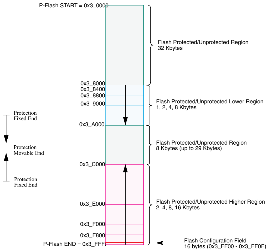
Figure 26-2. P-Flash Memory Map
