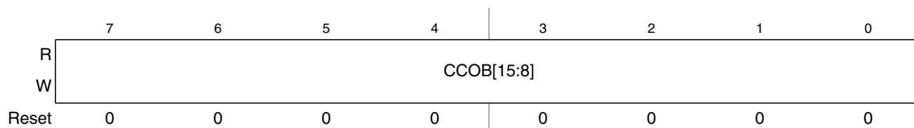
Figure 23-15. Flash Common Command Object High Register (FCCOBHI)
