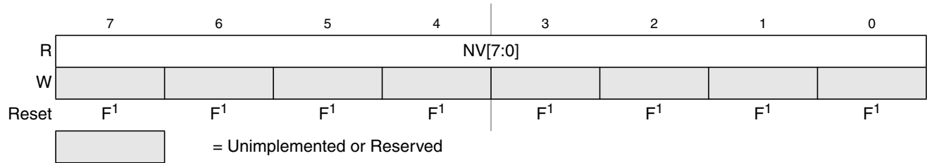
Figure 23-21. Flash Option Register (FOPT)
