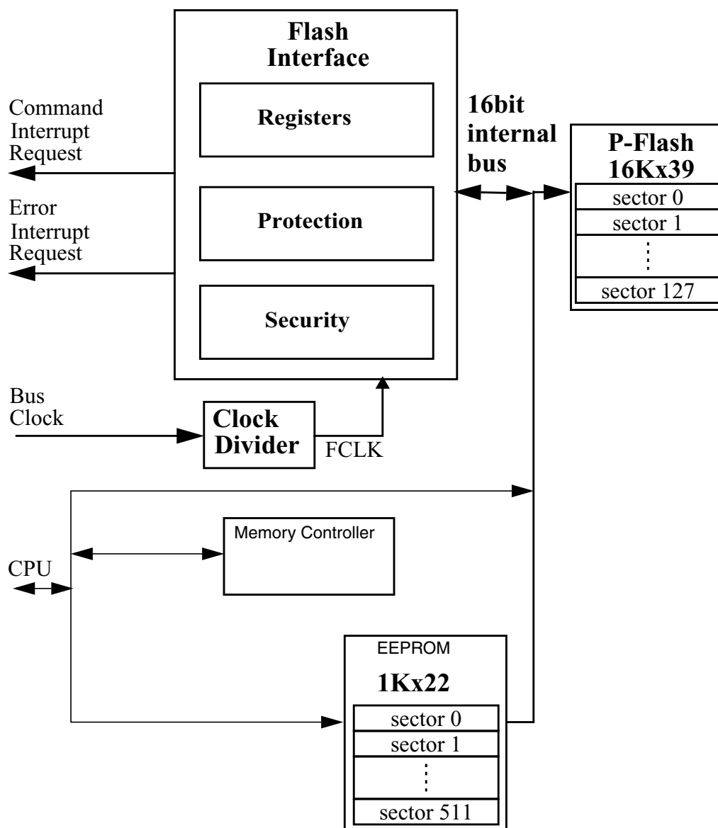
Figure 26-1. FTMRG64K1 Block Diagram
