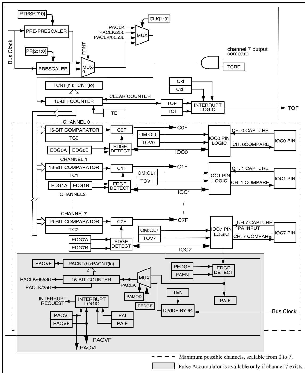
Figure 22-30. Detailed Timer Block Diagram
