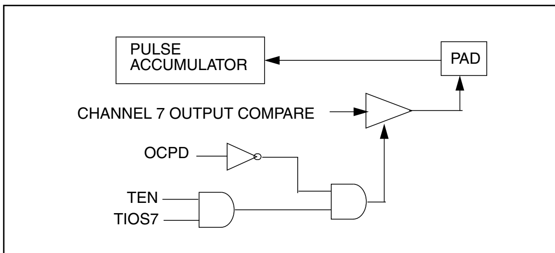
Figure 22-4. Channel 7 Output Compare/Pulse Accumulator Logic
