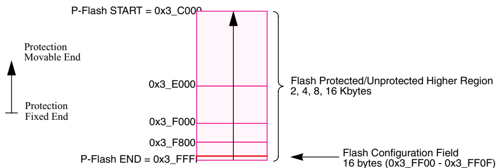
Figure 23-2. P-Flash Memory Map
