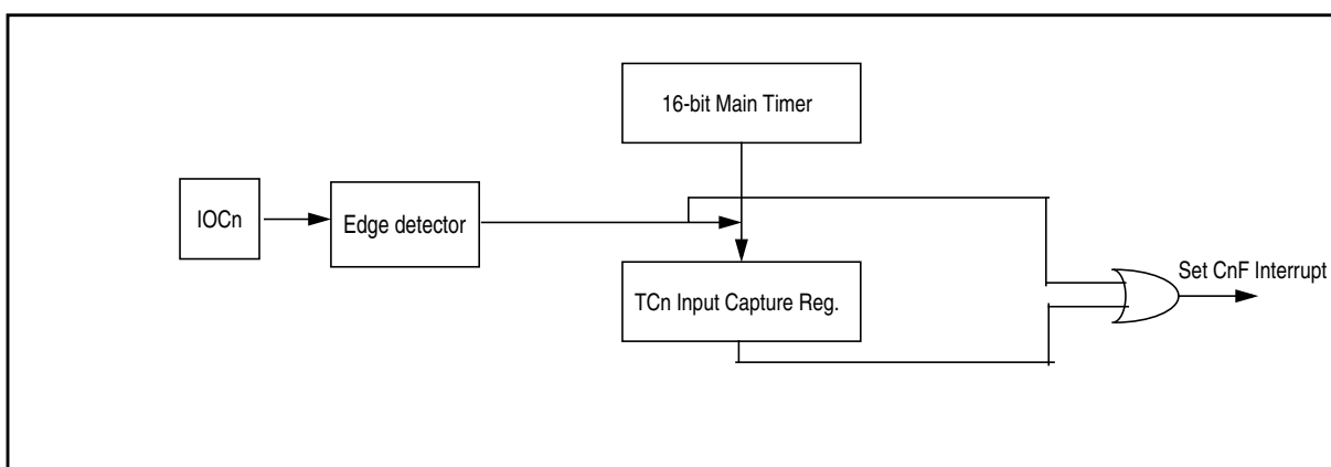
Figure 22-3. Interrupt Flag Setting
