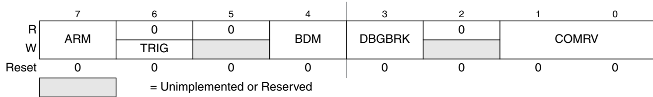
Figure 8-3. Debug Control Register (DBGCR1)
