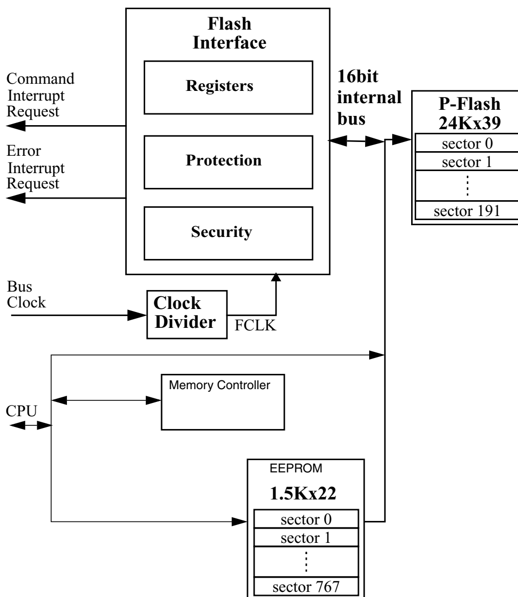
Figure 27-1. FTMRG96K1 Block Diagram
