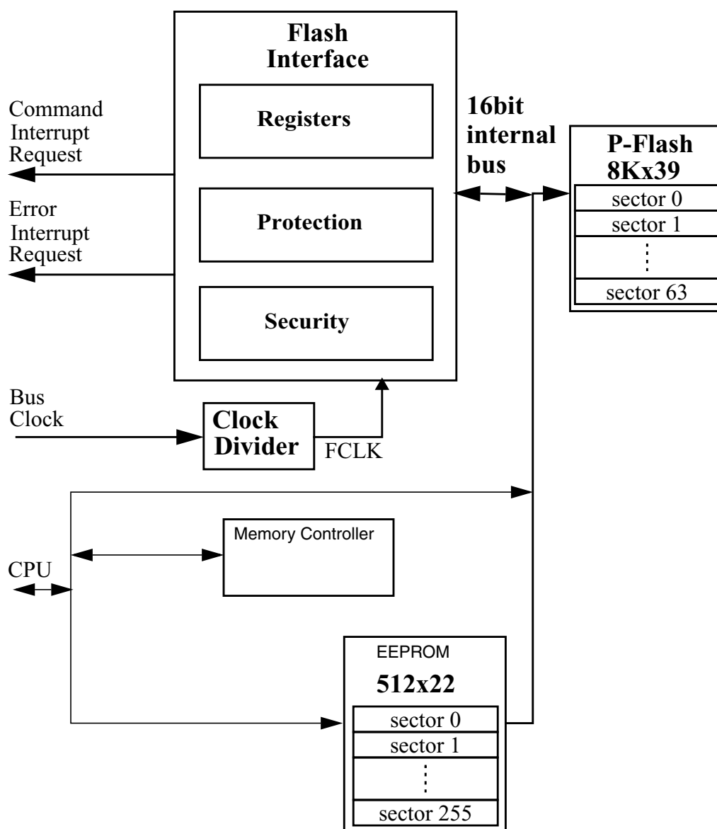
Figure 24-1. FTMRG32K1 Block Diagram
