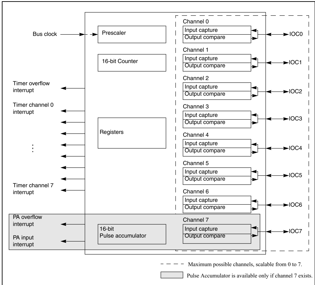
Figure 22-1. TIM16B8CV3 Block Diagram
