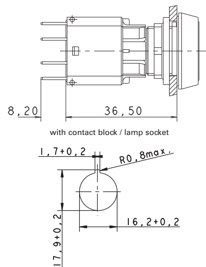
Panel cut-out
