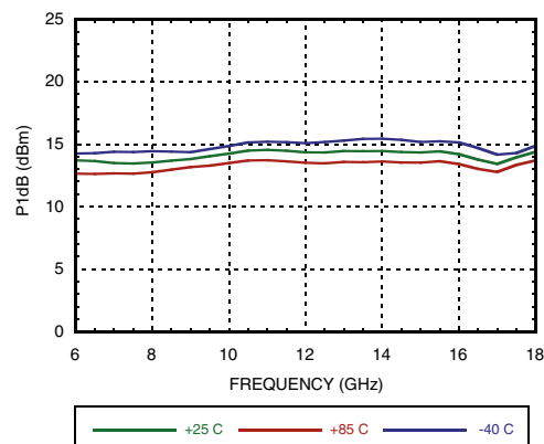
P1dB vs. Temperature [1]
