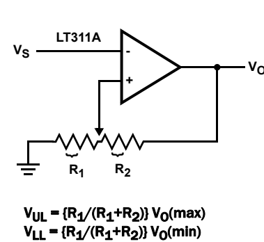
FIGURE 10. COMPARATOR WITH HYSTERESIS
