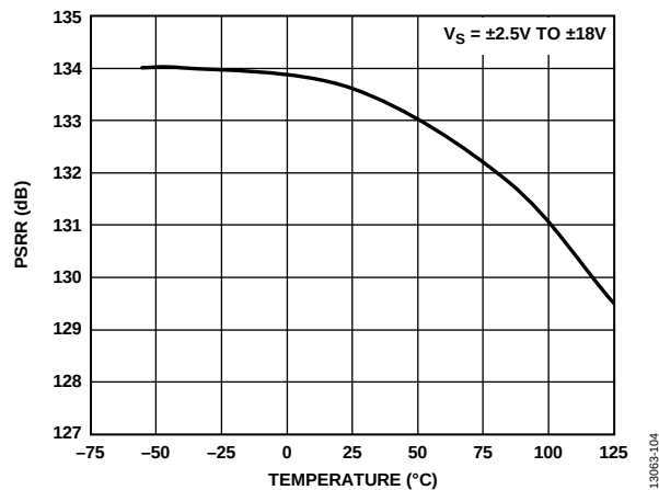
Figure 5. PSRR vs. Temperature
