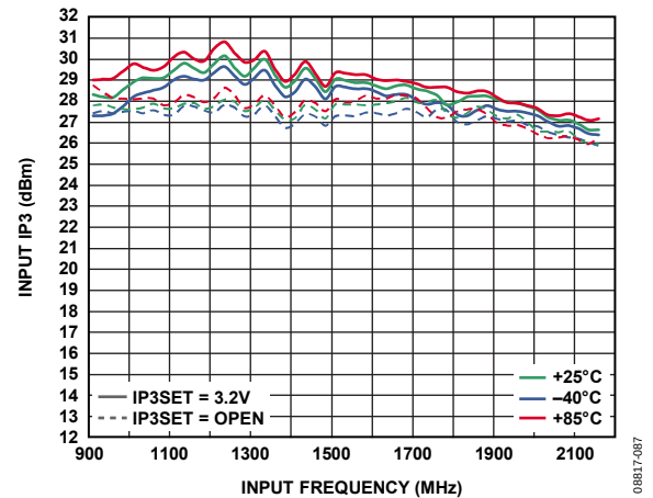
Figure 7. Input IP3 vs. Input Frequency
