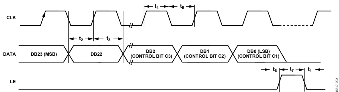
Figure 2. Timing Diagram
