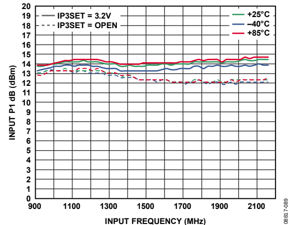
Figure 9. Input P1dB vs. Input Frequency
