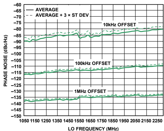
Figure 30. 25°C Spot Phase Noise vs. LO Frequency
