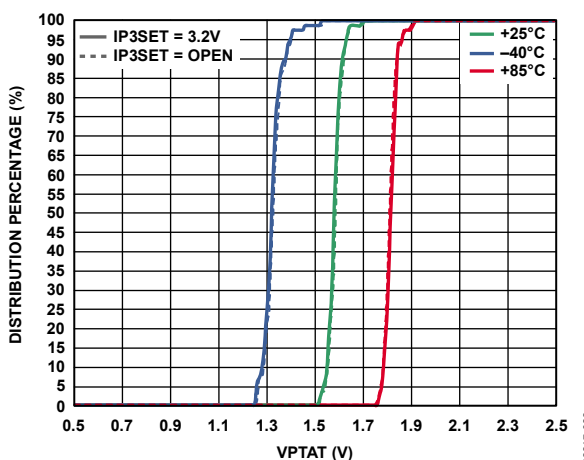
Figure 42. VPTAT MUXOUT Voltage
