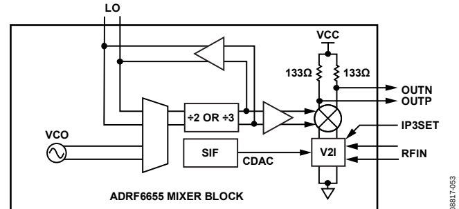
Figure 51. Mixer Block
