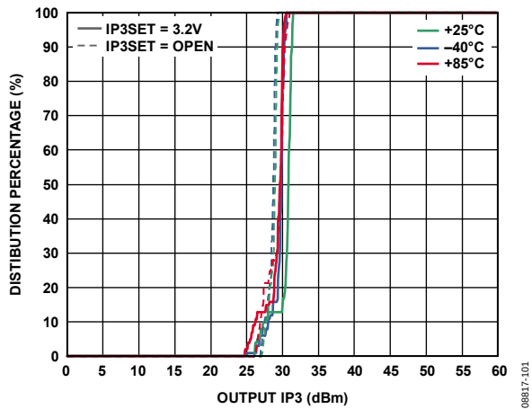
Figure 44. Output IP3 CCDF, LO = 1220 MHz, RF = 340 MHz
