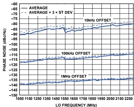
Figure 29. -10°C Spot Phase Noise vs. LO Frequency
