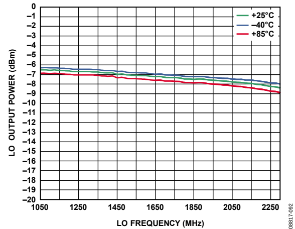
Figure 14. LO Port Output Power vs. LO Frequency
