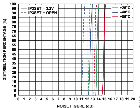
Figure 41. Rx Noise Figure CCDF
