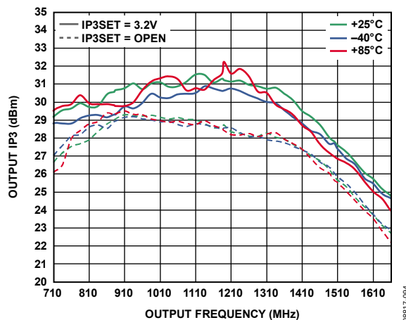
Figure 19. Output IP3 vs. Output Frequency
