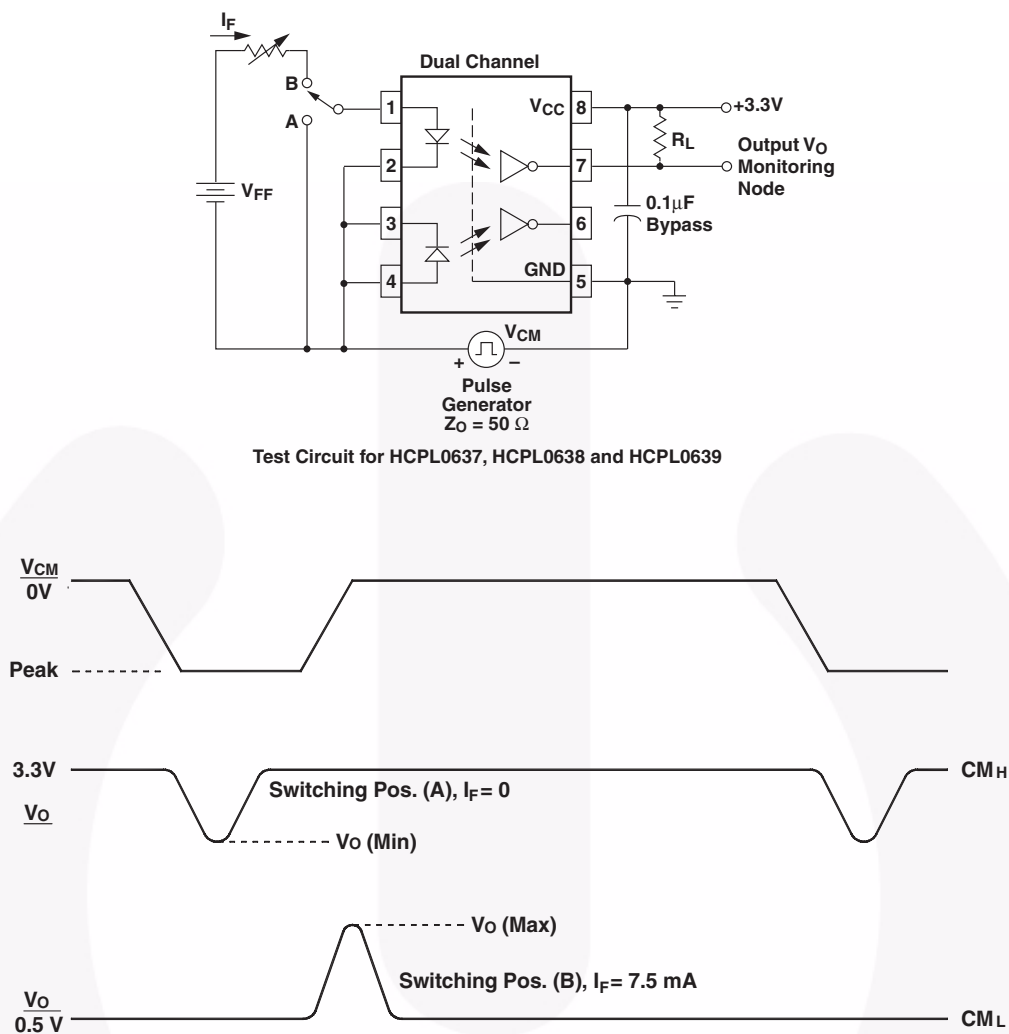
Fig. 23 Test Circuit Common Mode Transient Immunity (HCPL0637, HCPL0638 and HCPL0639)
