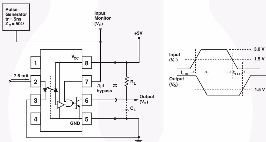
Fig. 21 Test Circuit t_{EHL} and t_{ELH} .
