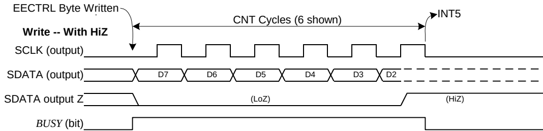
Figure 11: 3-wire Interface. Write Command, HiZ=1
