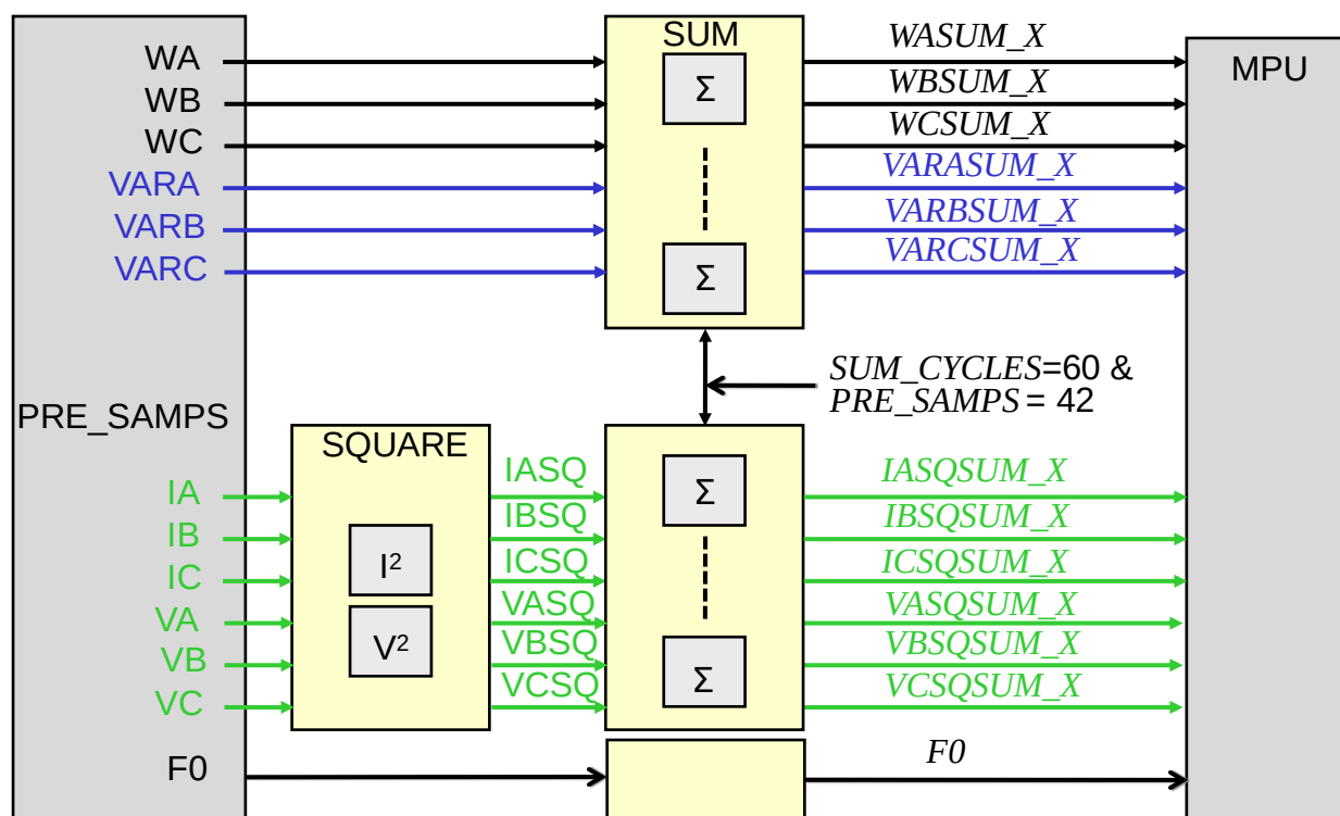
Figure 47: CE Data Flow: Squaring and Summation Stages
