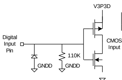
Digital Input
