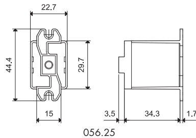
Rear flange mount adaptor for 55.32, 55.33, 55.34
