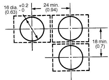
Panel cutout (top view)
