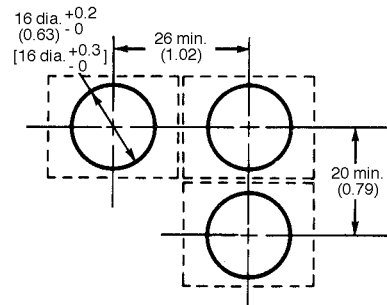
Panel cutout (top view)
