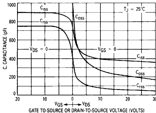
Figure 14. Capacitance Variation
