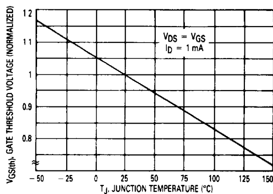
Figure 3. Gate-Threshold Voltage Variation With Temperature
