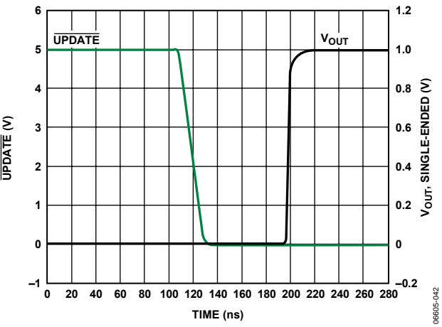
Figure 44. Enable Time
