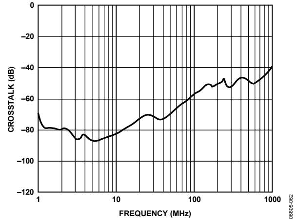
Figure 29. Crosstalk, All Hostile
