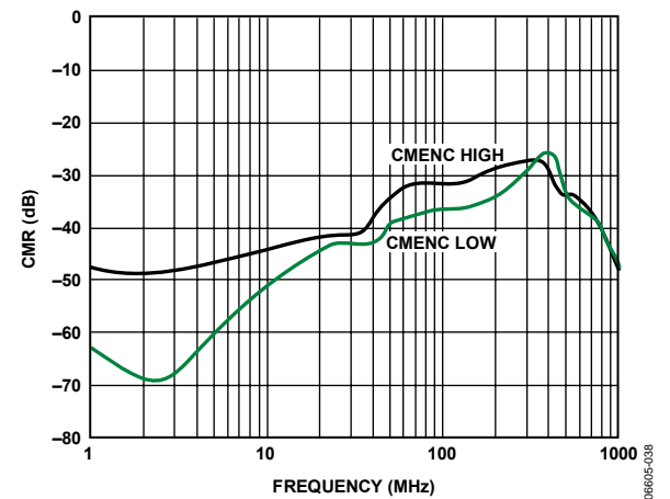
Figure 31. Common-Mode Rejection
