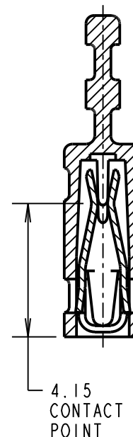
SECTION Y-Y
